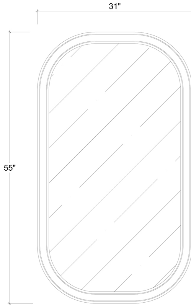
FRONT VIEW
