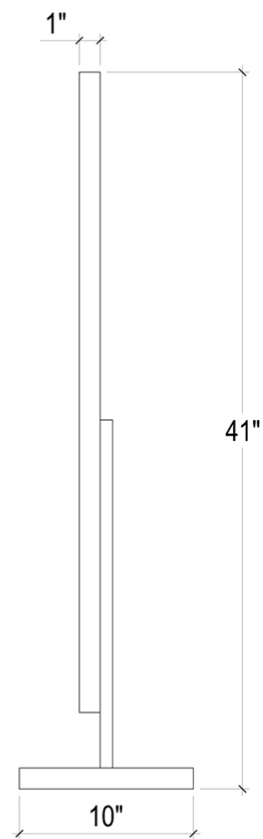
SIDE VIEW
